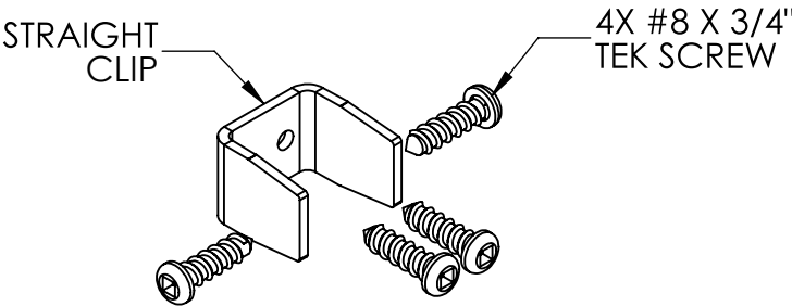
4X CLIP DETAIL
